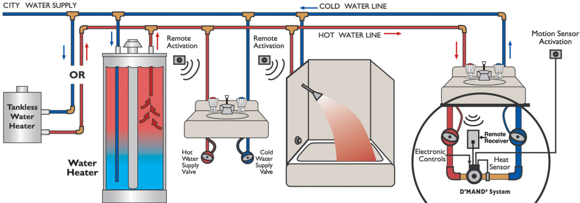
D'MAND® System for Standard Piping (Non-ReCirc)
